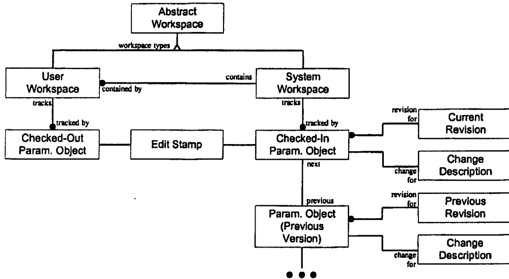
Figure 51 - Version Control Object Model
